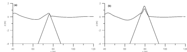
Figure 2 - Wave transmission over (left) and through (right) a breakwater with (a) and without (b) overtopping.
