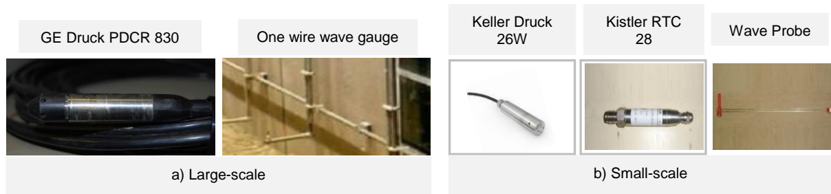
Figure 2. Large-scale (a) and Small-scale (b) instrumentations for measuring pressure and wave elevation.
