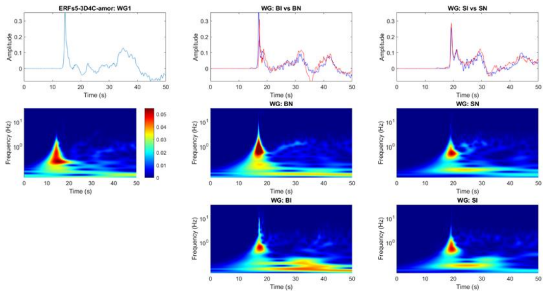
Figure 4. Time series of surface elevation (first row) and corresponding spectrograms (second and third row) of ERF5s in 8-LOS at WG1 (first column), BN & BI (second column), and SN & SI (third column)
