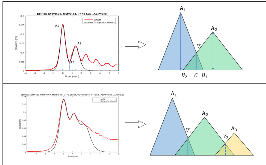
Figure 5. The overlapped waves simplified into two or three isosceles triangles; red solid line: time series of data of ERF8s (above) and ERF12s (below), black dash-dot line: overlapped solitary wave, A: amplification of solitary wave, V: minimum elevation between two near crests.
