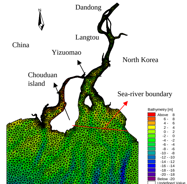
Model Computational Grid
