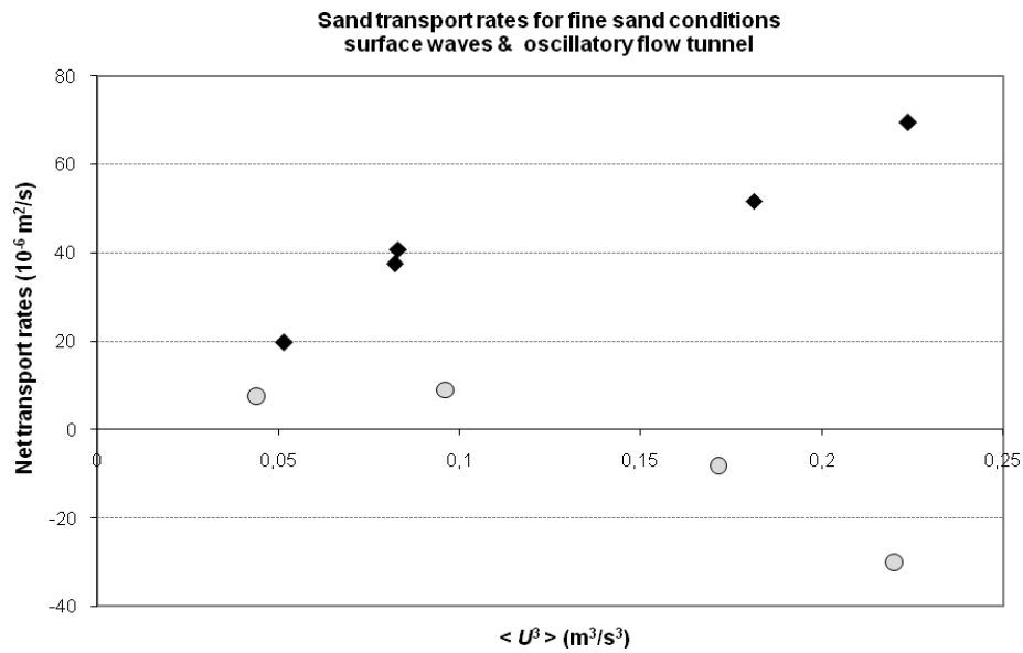
Figure 9. Measured sand transport rates for fine sand conditions from i) new flume experiments (black diamonds) and ii) oscillatory flow tunnel experiments (open circles) (Ribberink & Chen, 1993; O'Donoghue & Wright, 2004b).
