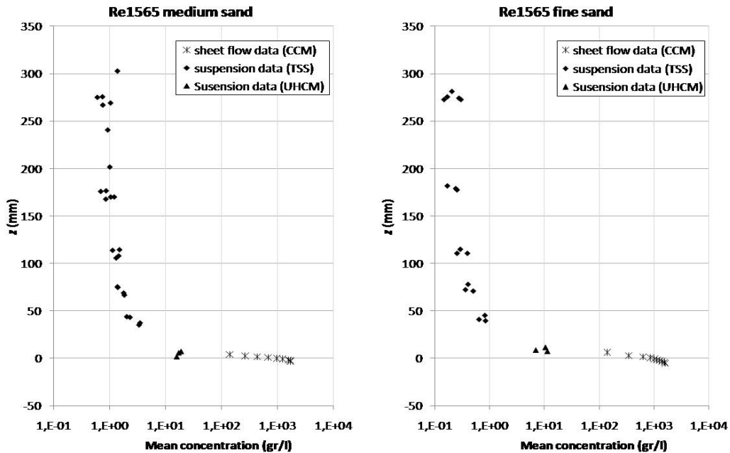
Figure 4. Time averaged concentration profiles (both suspension and sheet flow layer) for condition Re1565 for medium and fine sand conditions.
