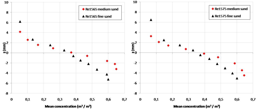
Figure 5. Time averaged sheet flow layer concentration profiles for wave conditions Re1565 (left graph) and Re1575 (right graph), for both medium (red diamonds) and fine (black triangles) sand conditions.
