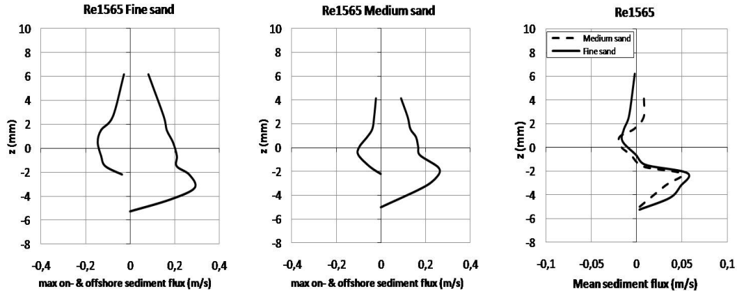
Figure 6. Vertical profiles of the measured sediment fluxes for Re1565. Left graphs: fine sand maximum on- and offshore profiles results. Middle graphs: medium sand maximum on- and offshore profiles results. Right graphs: mean sediment fluxes for medium and fine sand.
