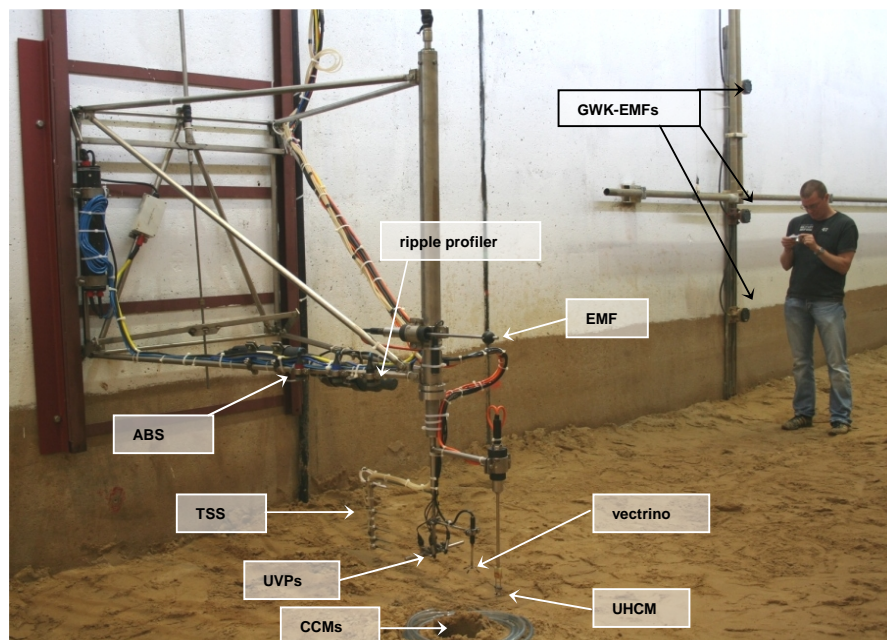
Figure 2. Overview of the wall frame with instruments mounted in the Large Wave Flume. The CCM-tank is buried underneath the sand bed. Three additional EMFs are attached to the wall, close to the frame.
