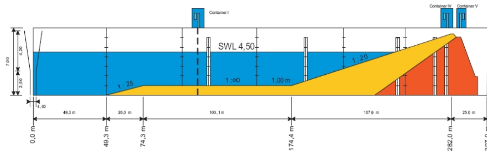
Figure 1. Overview of the Large Wave Flume of the Coastal Research Centre, Hannover, Germany.
