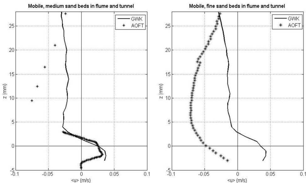
Figure 3. Mean flow velocity measurements inside the wave boundary layer under full scale surface waves (GWK) and oscillatory flow (AOFT) for medium (left graph) and fine (right graph) sand conditions (oscillatory flow tunnel results after Ribberink et al., 2008 and Campbell et al., 2006).
