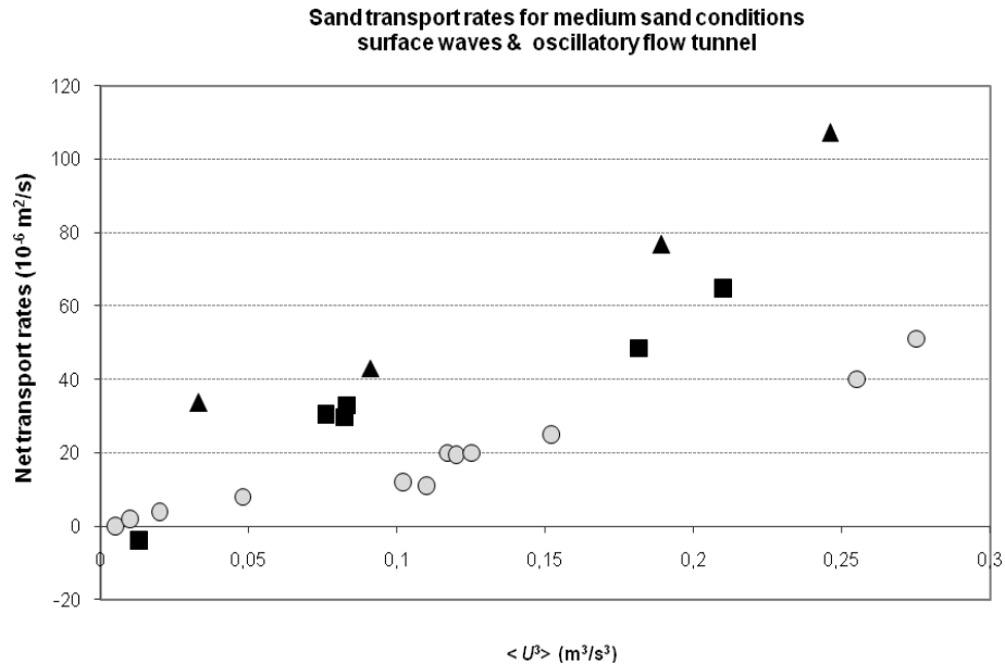
Figure 8. Measured sand transport rates for medium sand conditions from i) new flume experiments (black squares), ii) previous flume experiments (black triangles) (Dohmen-Janssen & Hanes, 2002) and iii) oscillatory flow tunnel experiments (open circles) (Ribberink & Al Salem, 1994; Hassan & Ribberink, 2005).
