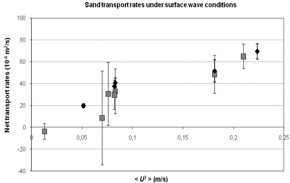
Figure 7. Measured sand transport rates versus third-order velocity moment for both medium sand (grey squares) and fine sand (black diamonds) conditions.
