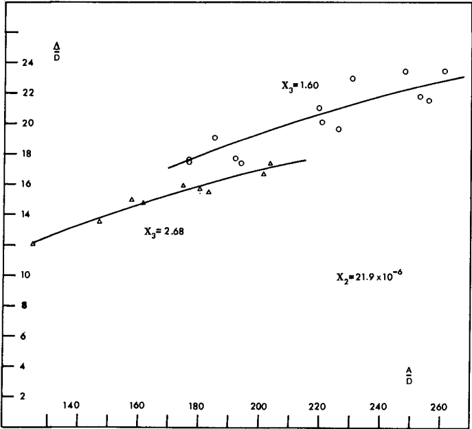
FIG.6 VARIATION OF \Delta/D WITH X_2 = \rho_2/\rho
