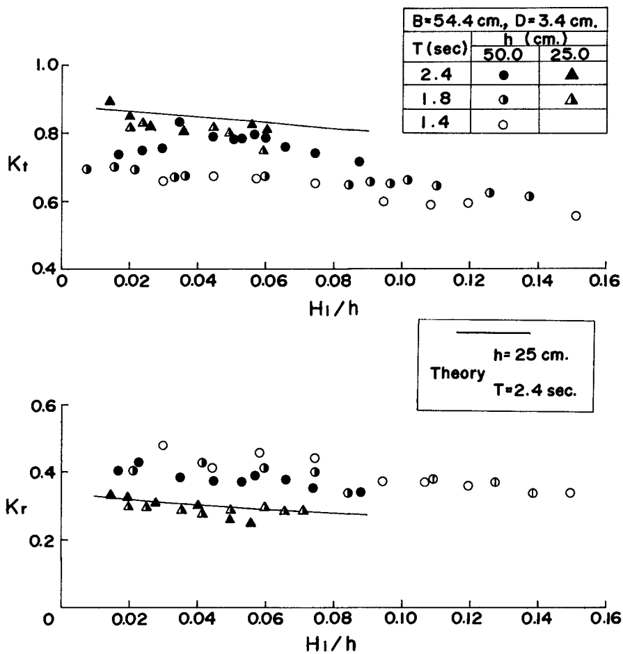
Fig.-5 K_t & K_r versus H_l/h (Horizontal Bottom)
