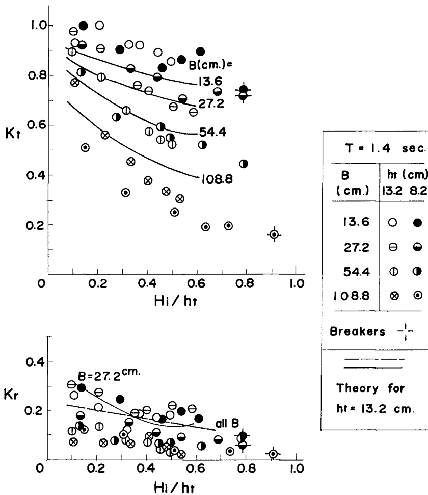
Fig.-6 K_t & K_r versus H_i/h_t ( 1/40 Sloping Bottom )
