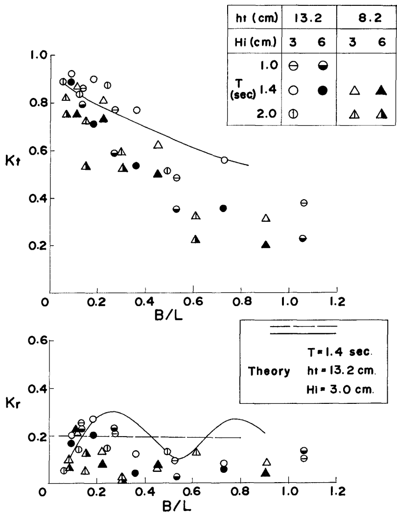
Fig.-8 K_t & K_r versus B/L ( 1/40 Sloping Bottom )
