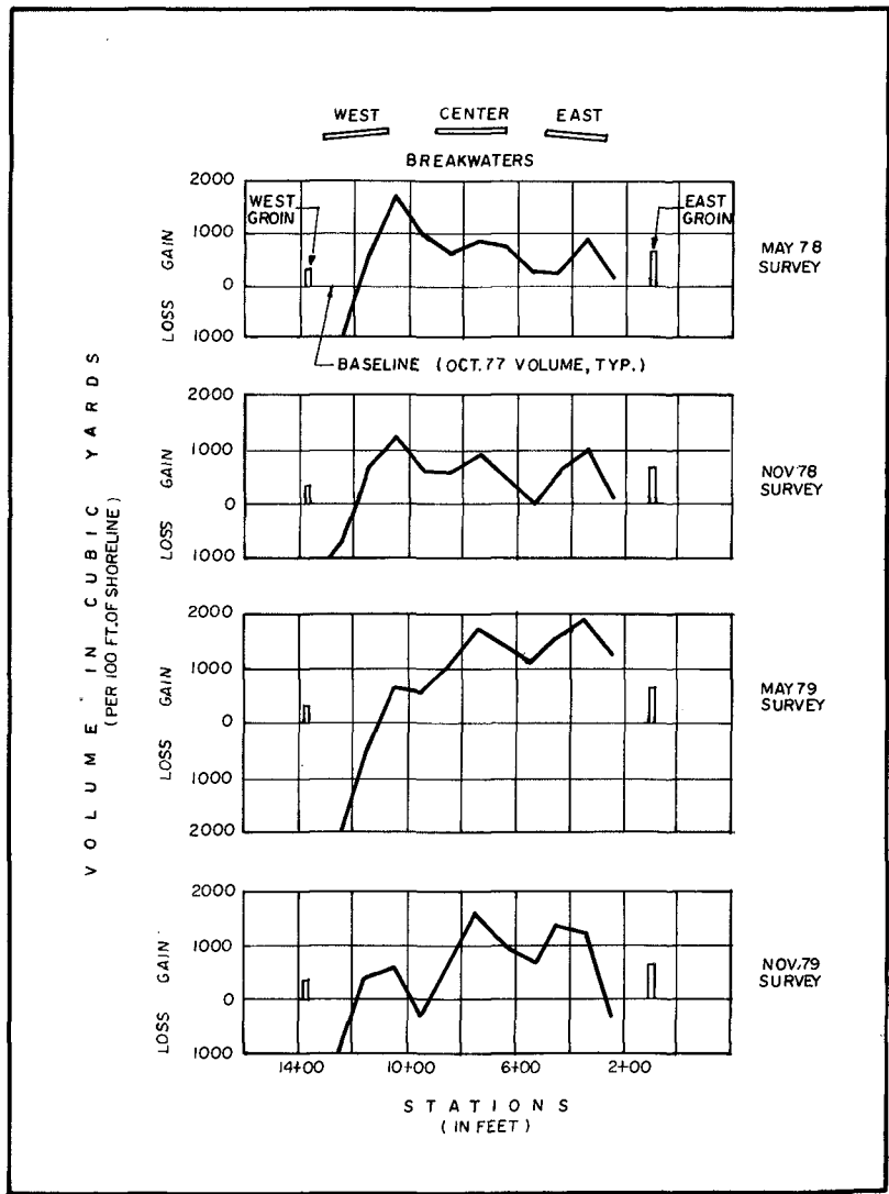
FIGURE 12: SAND VOLUME CHANGES RELATIVE TO OCTOBER 1977
