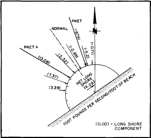
FIGURE 4: ENERGY-FLUX P_s AT THE PROJECT SITE
