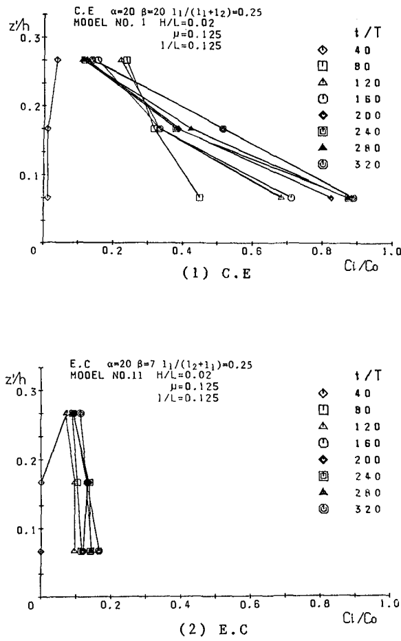
Fig.9 Vertical concentration distribution at regular time intervals
