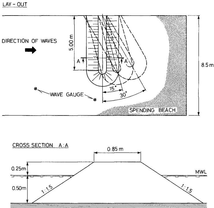
Fig 2. Lay-out and cross section of the model. (Continued on next page).
