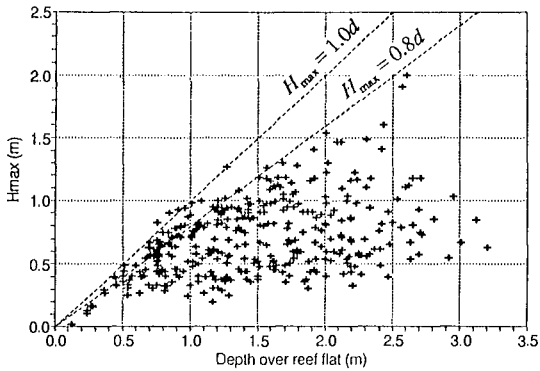
Figure 14. Maximum wave height vs water depth over reef, ZP2
