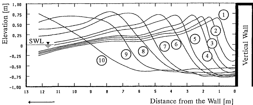
Fig. 4. Wave Profiles in Front of a Vertical Wall at Different Time Steps
