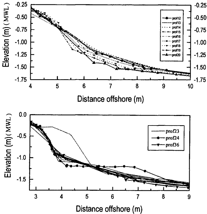
Fig. 3. Beach face steepening and scarp generation (ST_10).
