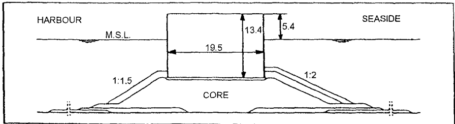
Figure 7 Cross section caisson breakwater
