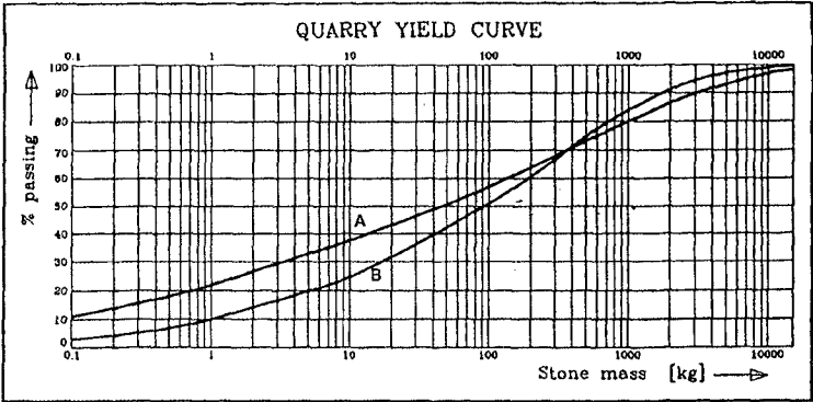
Figure 3 Quarry yield curves
