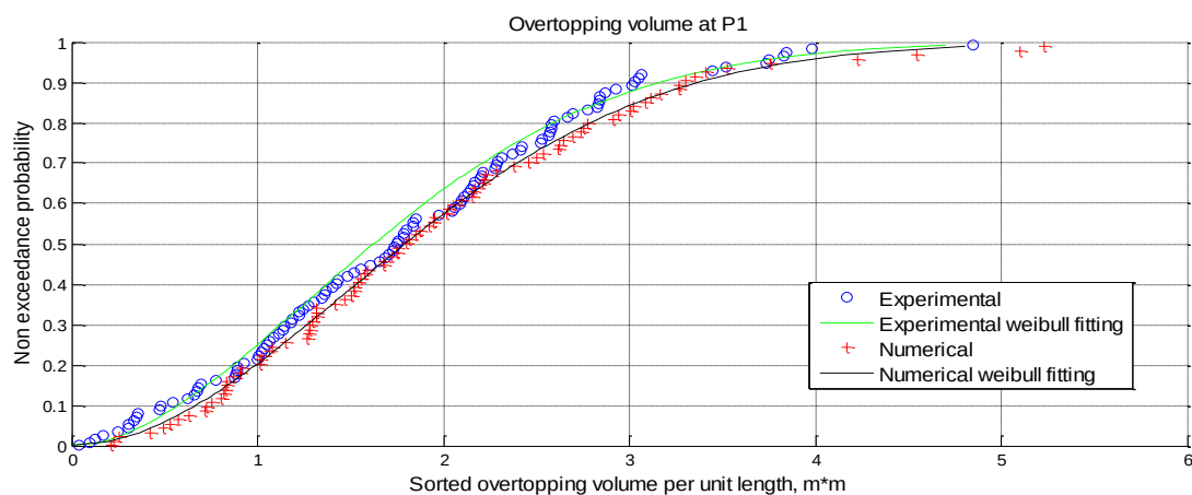
Figure 7. Test R14 (test without structure): comparison of computed and measured overtopping volumes at gauge P1.
