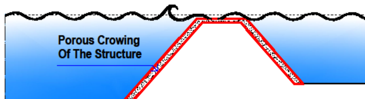
Figure 8. Geometrical scheme for the test with a single porous layer.
