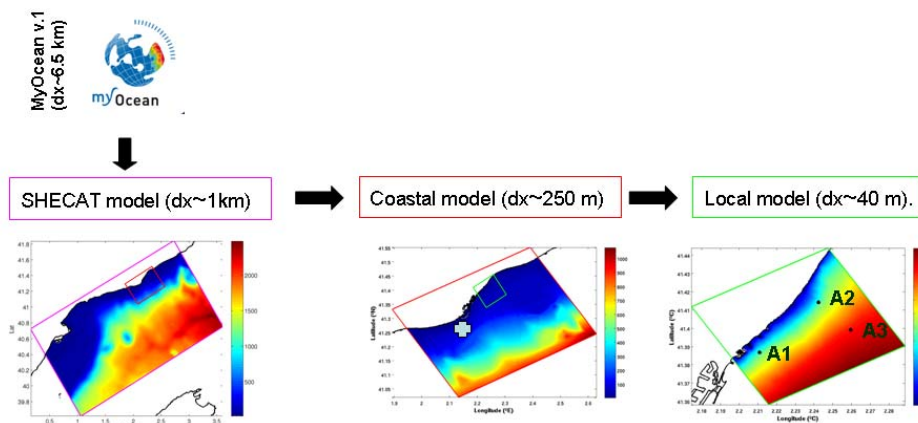
Figure 4. Nested modeling sequence developed for the Catalan coast. It is linked to the MyOcean operational system that provides the offshore boundary conditions for the currents. The bathymetry and numerical domains correspond to the domains denoted as SHECAT (shelf), COASTAL (inner shelf) and LOCAL (nearshore, including the surf zone). The ADCP sensor locations are shown in the figure (A1, A2 and A3) and also de Llobregat buoy from the XIOM network (cross symbol).
