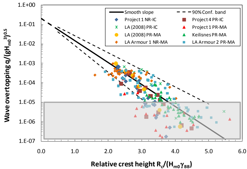
Figure 11. Wave overtopping for none and partly reshaping berm breakwaters.
