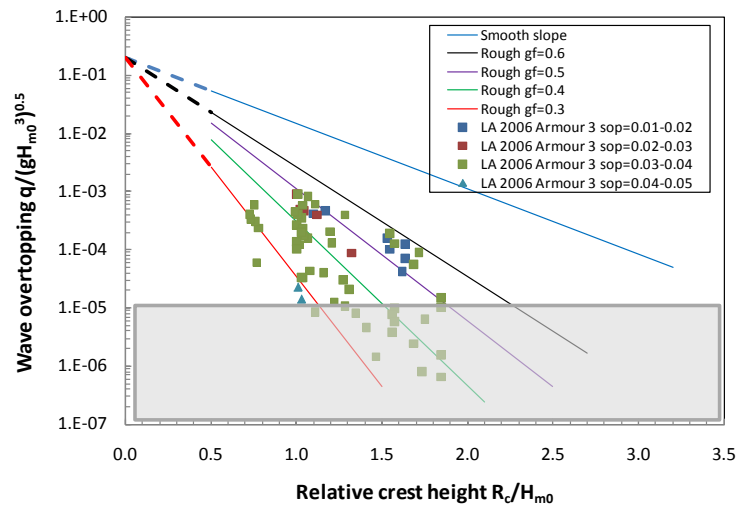
Figure 5. Wave overtopping for Lykke Andersen (2006), armour 3, FR MA.
