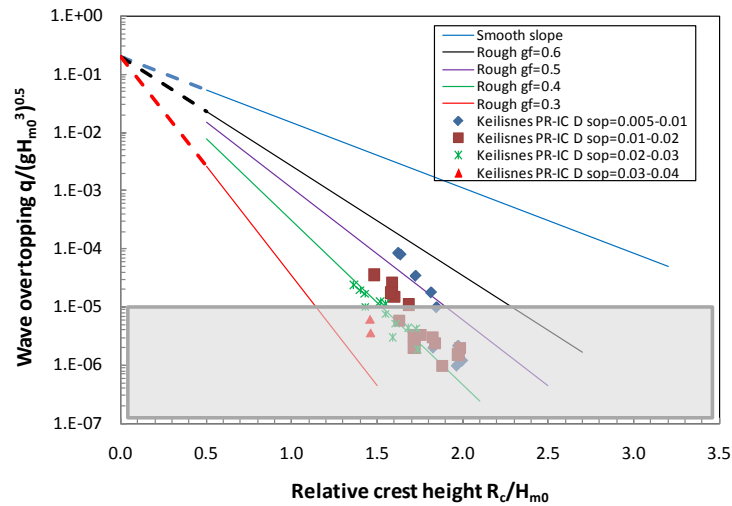
Figure 4. Wave overtopping for Keilises, PR IC.
