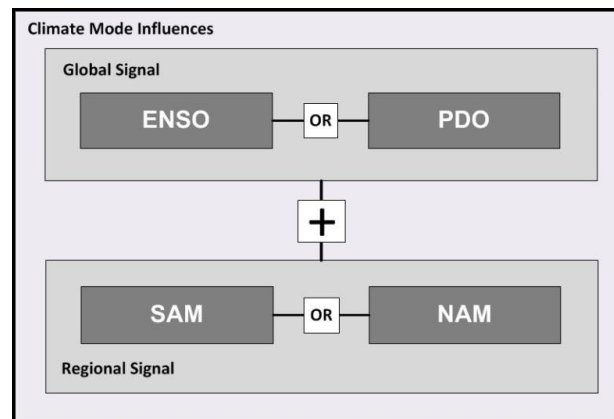
Figure 4. Schematic representation of climate mode component.
