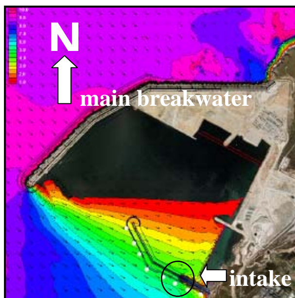
Figure 1. Wave agitation in the Punta Langosteira harbor after the construction of the main breakwater.
