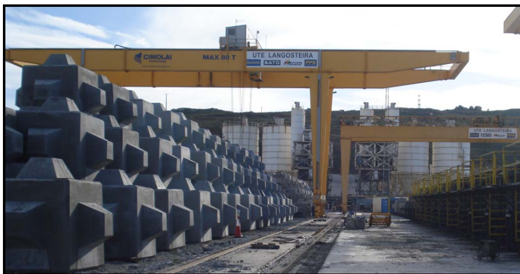
Figure 6. Block yard, gantry cranes and stacking of 15-tonne and 25-tonne Cubipod units in three levels.
