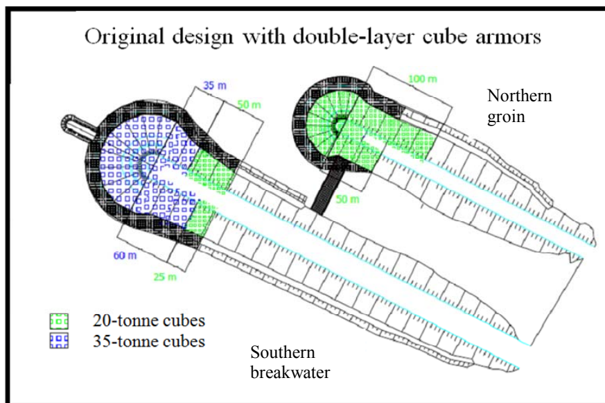
Figure 2. Original design with conventional H/V=2.0 and 1.75 slopes, double-layer 35-tonne and 20-tonne cube armors.
