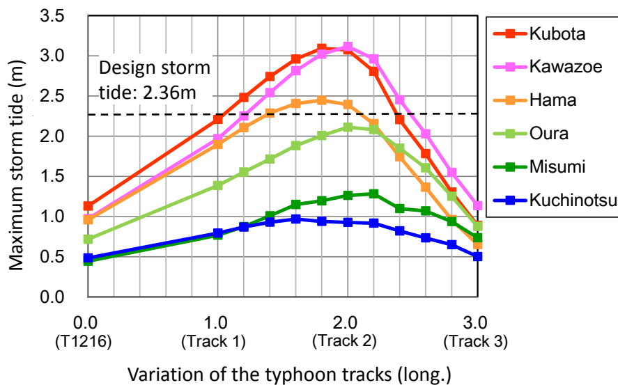
Figure 14. Changes of the maximum storm tides dependent on the typhoon tracks.
