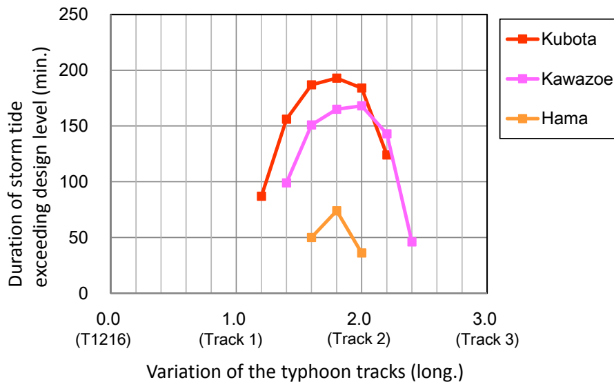
Figure 15. Changes of the duration in which the storm tide exceeds the design storm tide dependent on the typhoon tracks.
