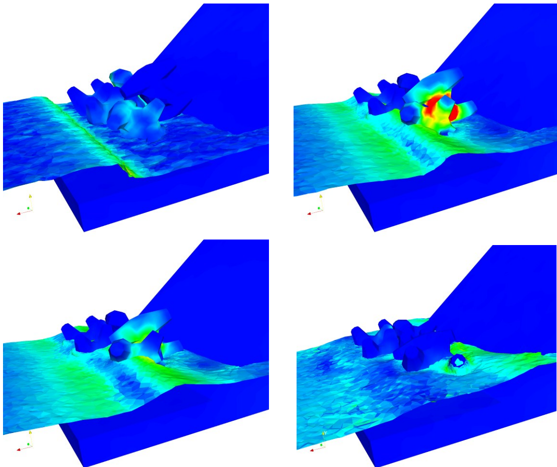
Figure 16 Two-way coupled motion of five CORE-LOC™ concrete units falling through water, with gravitational acceleration, modelled with Y3D/Fluidity (Xiang et al., 2013).
