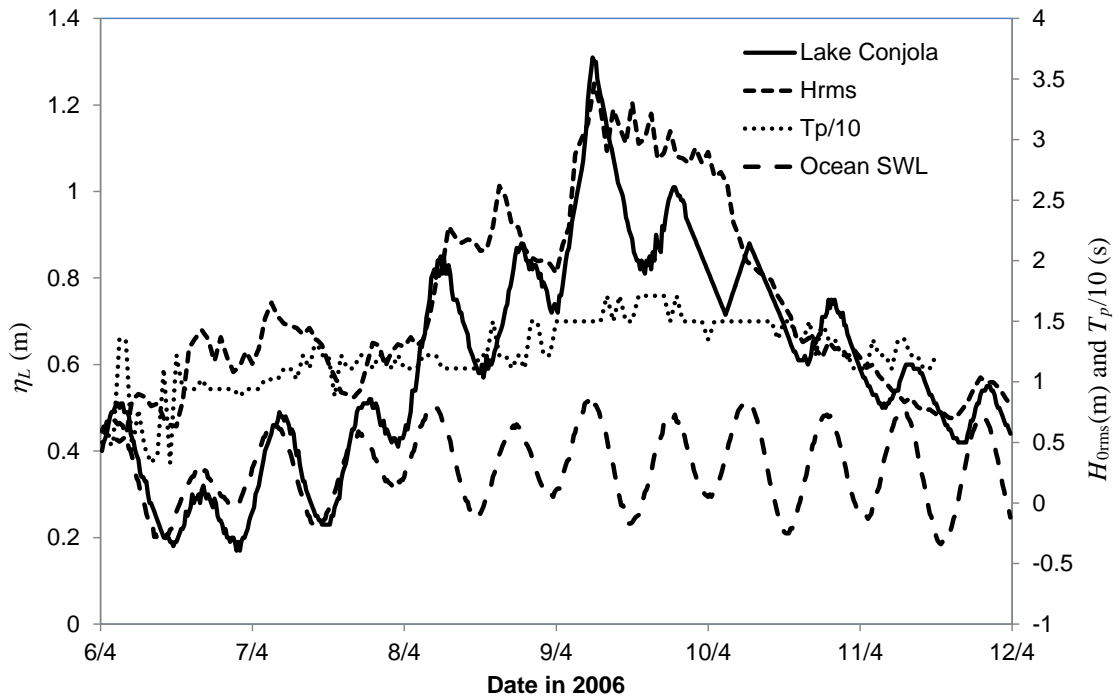
Figure 2—Lake Conjola water surface level near the caravan park ( \eta_L , continuous line, left axis), the offshore root mean square wave height ( H_{0rms} , short dashed line, right axis), peak wave period ( T_p , dotted line divided by 10, right axis) and ocean surface level (long dashed, left axis) for April 2006 flooding.
