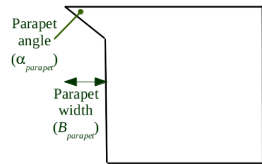
Figure 6: Definition sketch for the main parameters of the deflecting parapet (surge stopper)
