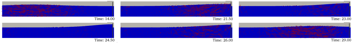
Figure 4: Tsunami approaching an impermeable TFB structure, results from CFD simulations for the VOF function (phase fraction) and vectors representing particle velocities, without overtopping ( d = 20m, H = 4m & f = 8m ).
