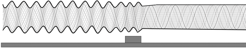
Figure 2: Envelope of free surface displacement around the submerged breakwater.
