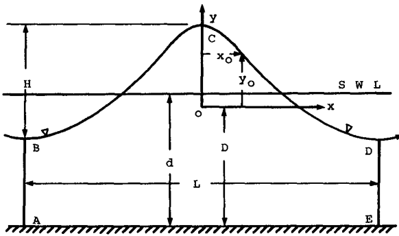
Fig 1 - The z-Plane
